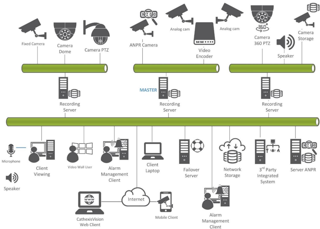
Figure 1: Site-based architecture
